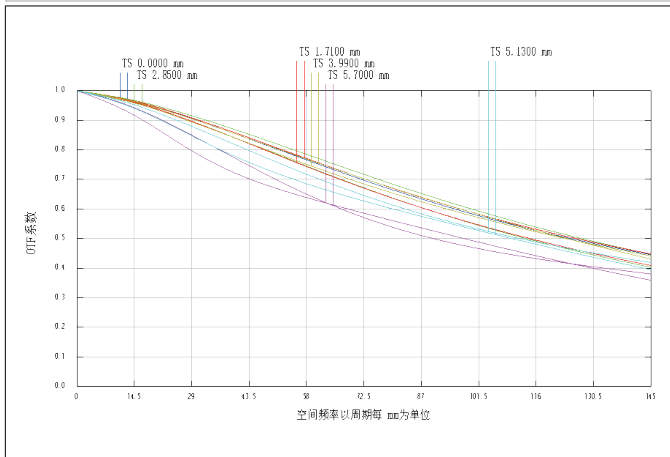
MTF
